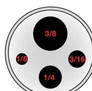
Multi-hole type 2 (CTC/MTC-320 A / 650 A)
