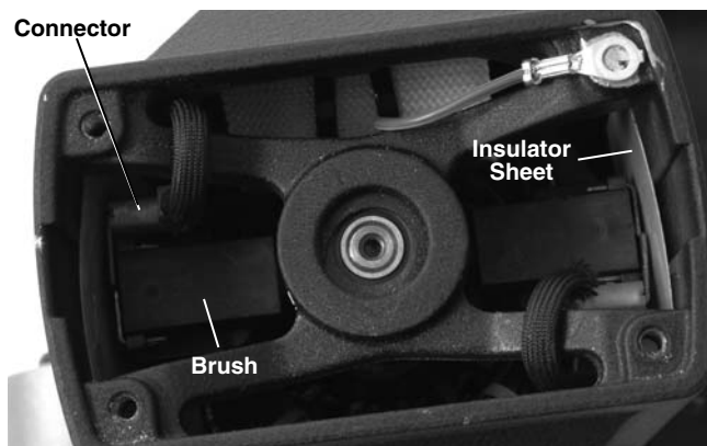
Figure 12 – Brush Placement - Motor Cover Removed
