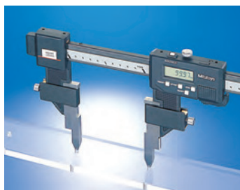
Centerline attachments
