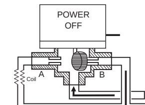
Figure-6f 3-Way Valve in Diverting Configuration Normally Open to the Coil.
