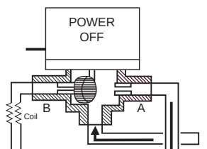
Figure-6e 3-Way Valve in Diverting Configuration Normally Closed to the Coil.
