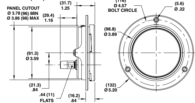
3½" 1009 Back Connect (XFF)
