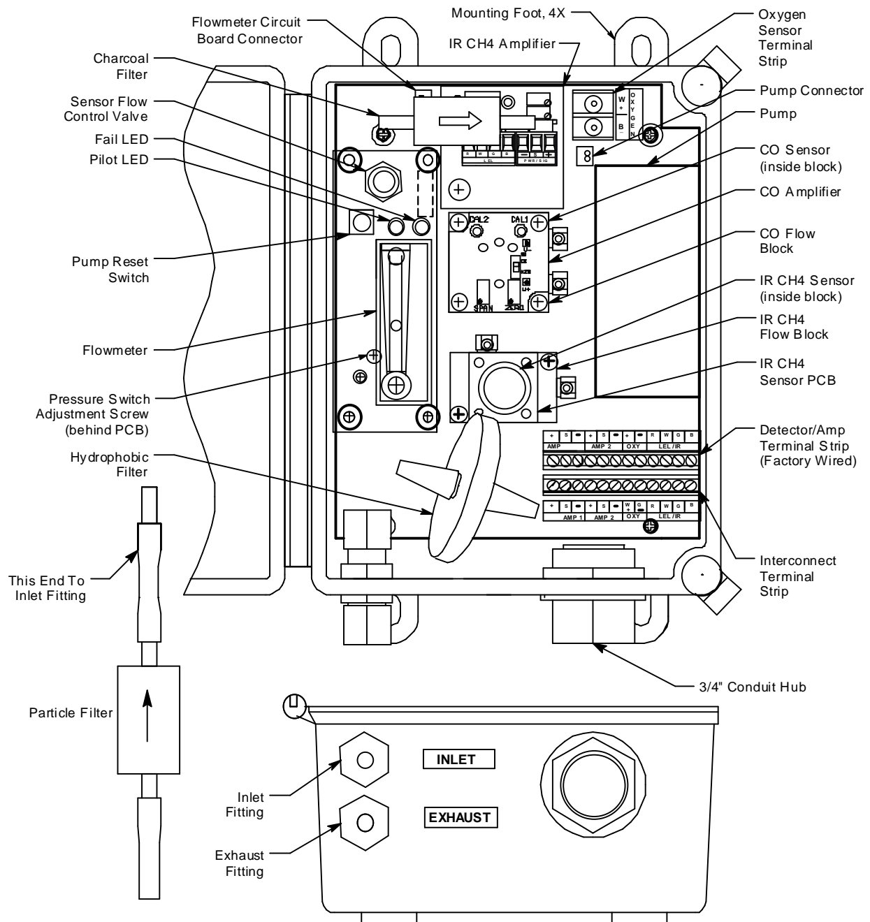
Figure 1: Methane/Carbon Monoxide Sample-Draw Detector Component Location
