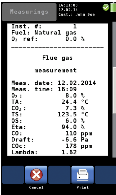
Fig. 34: Print Preview
