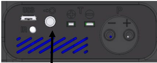
Fig. 50: Connector for the spillage probe at the bottom of the analyzer
