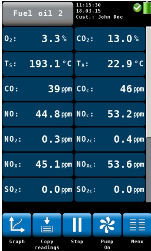
Fig. 18: Display details
