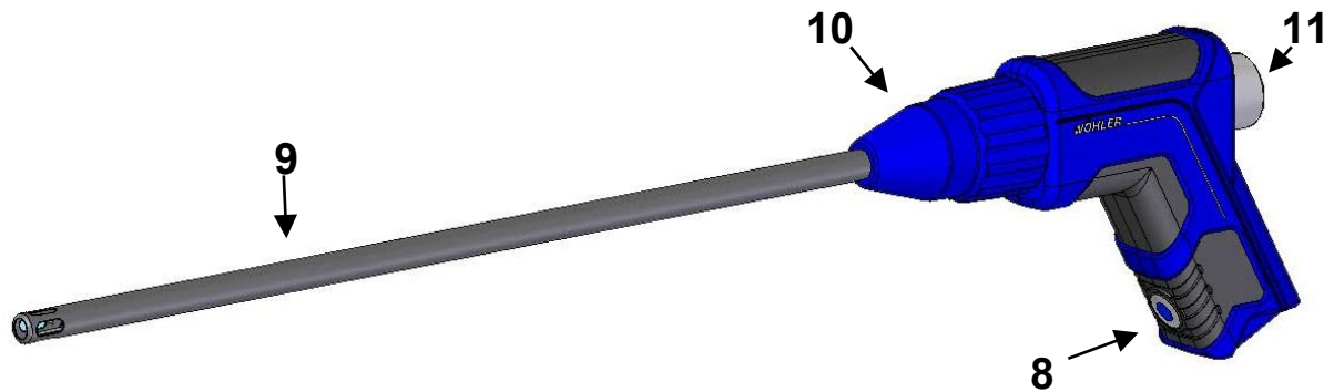
Fig. 4: Probe handle with gas probe 295 mm
