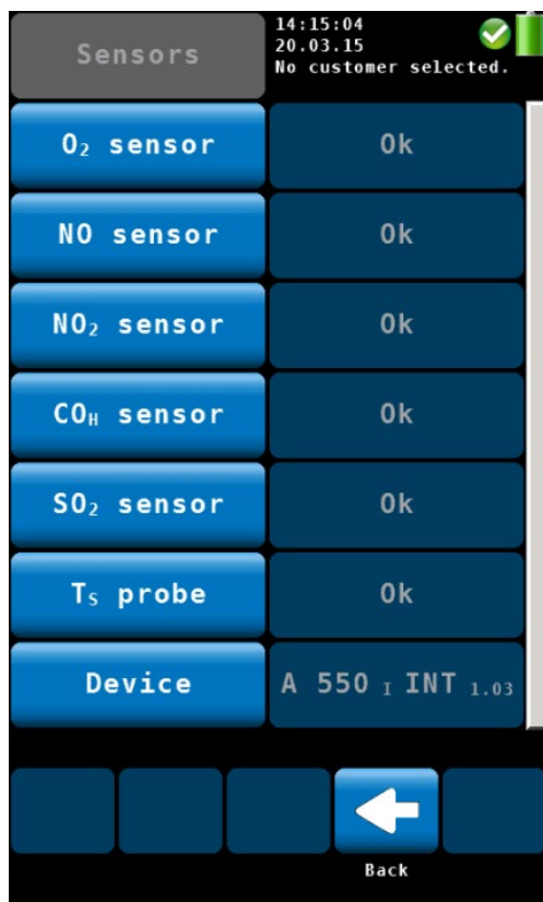
Fig. 71: Sensor diagnosis
