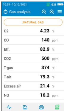
The probe can be inserted in the chimney. The analyzer displays the measurements.
