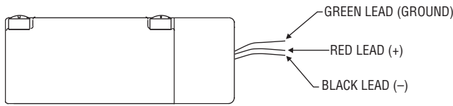
Figure 4 1/2" Conduit Connection
