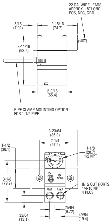
Figure 1 Pipe Mounting
