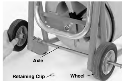
Figure 4 – Assembling Wheel
