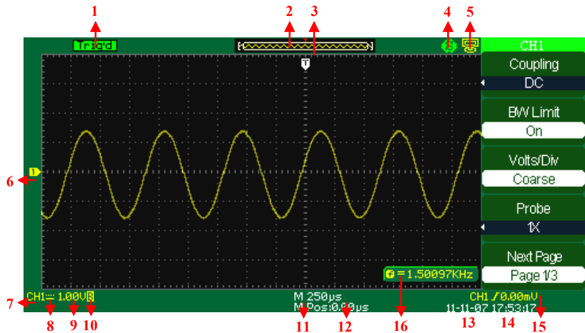
Figure 5 - Display Screen
