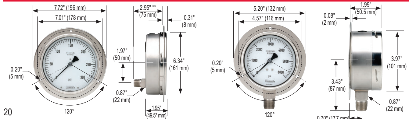
60-410/510 Front Flange
