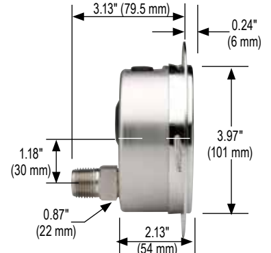
40-400/500 Rear Flange
