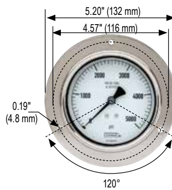
40-400/500 Rear Flange
