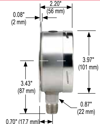
40-400/500 Rear Flange
