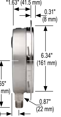
60-400/500 Front Flange
