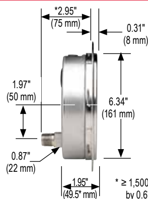
60-410/510 Front Flange
