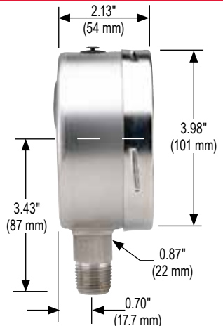
40-400/500
