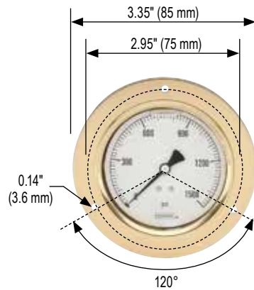
25-310 Front Flange
