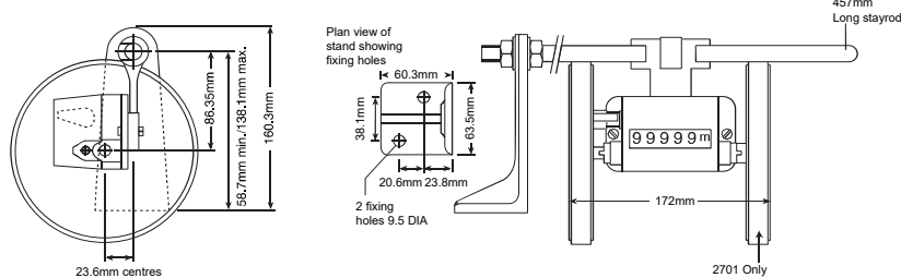
Product Dimensions 2401 | 2701
