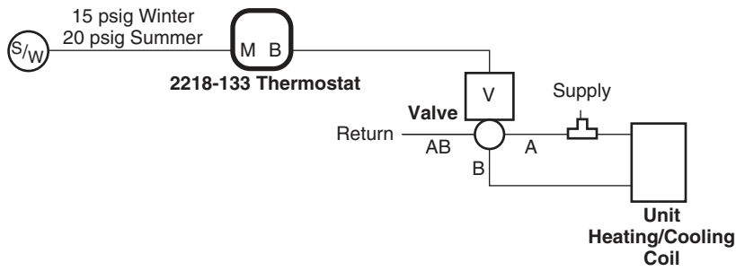
Figure 7 2218-133 Typical Application.
