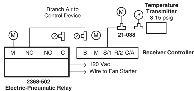
Figure 1 Typical Application.
