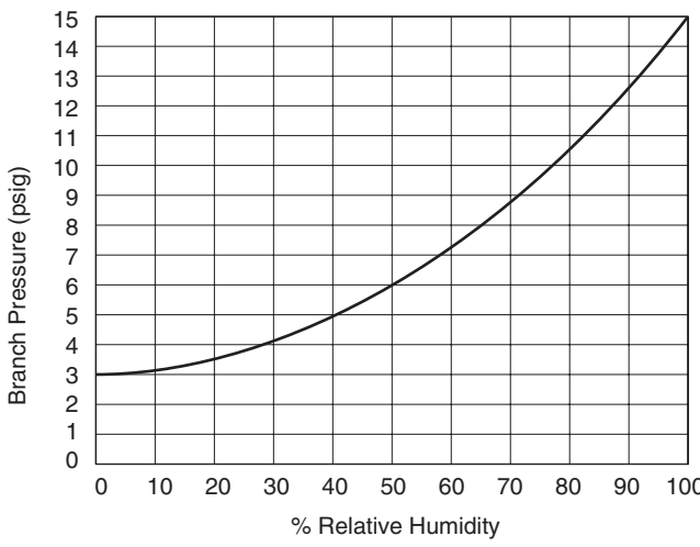
Figure 2 Relative Humidity vs. Branch Pressure.
