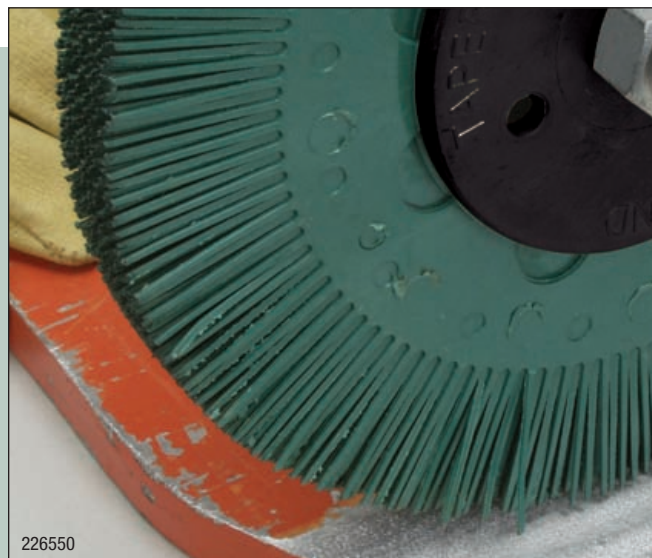
8" Radial Bristle Brush, grade 50, removing paint mounted on a straight shaft tool.
