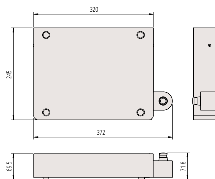
Electronic unit
