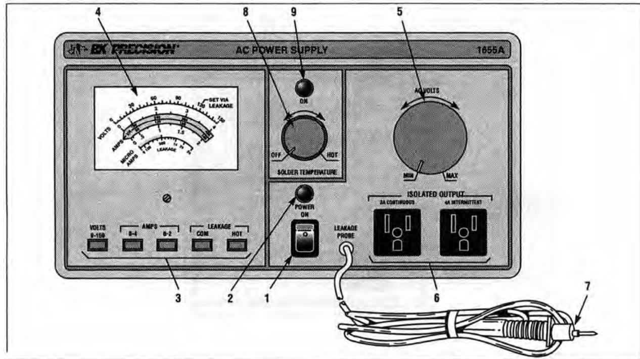
Figure 1. Front Panel Controls and Indicators, Model 1655A
