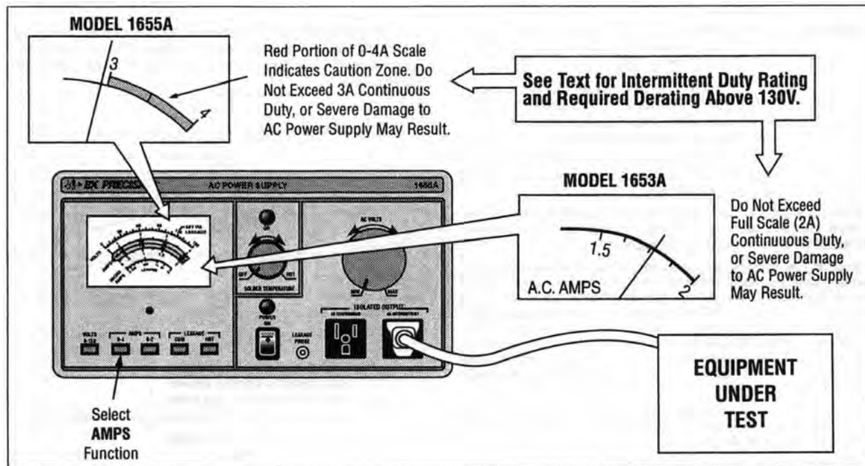
Figure 6. Maximum Current Considerations.
