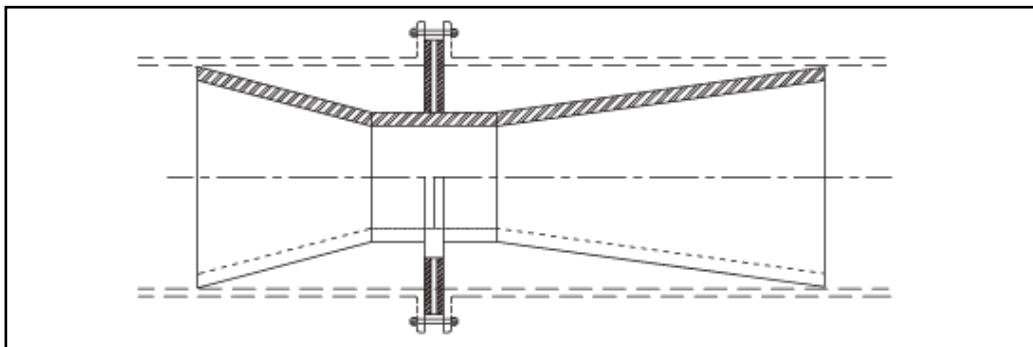
Fig 7: Insertion Type
