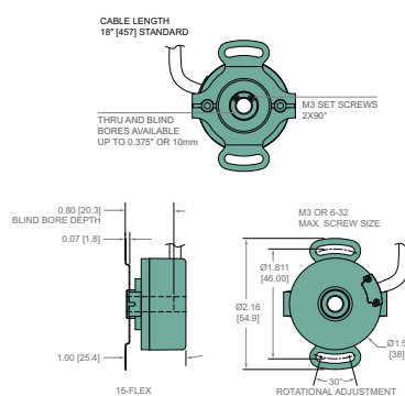
Model 15T/H 1.811" (46 mm) Slotted Flex Mount (SF)
