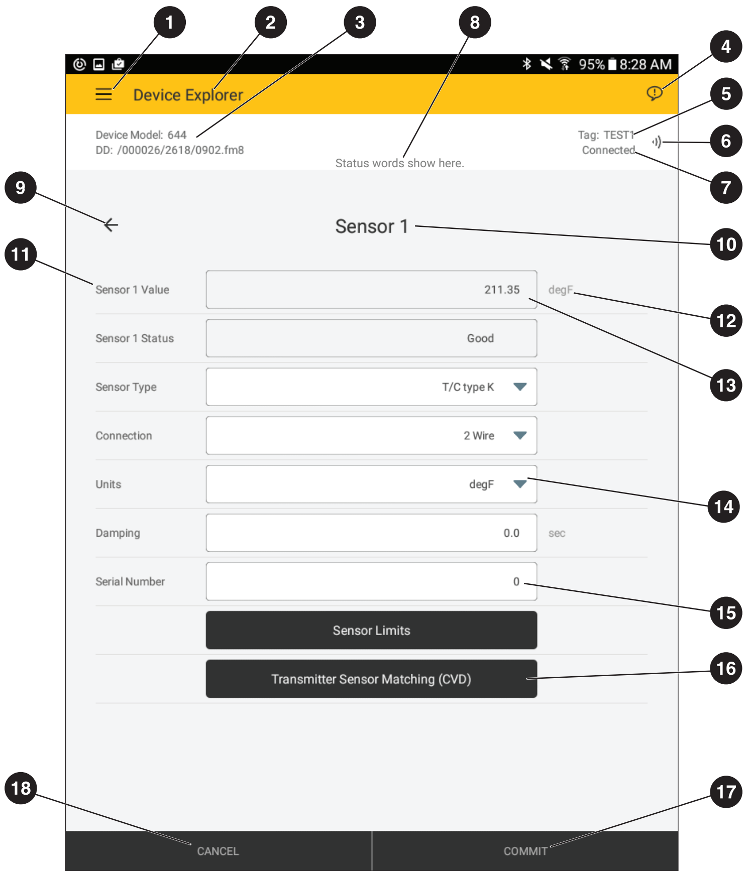
Figure 1. Sample Menu
