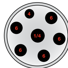
Multi-hole M02 (ATC-156/320/650 A/B / ITC-320/650 A)
