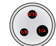
Multi-hole type 2 (CTC/MTC-140 A)
