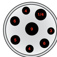
Multi-hole M04 (ATC-156/320/650 A/B / ITC-320/650 A)
