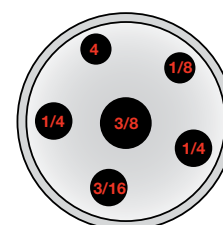
Multi-hole M06 (ATC-156/320/650 A/B / ITC-320/650 A)
