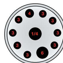
Multi-hole M03 (ATC-156/320/650 A/B / ITC-320/650 A)
