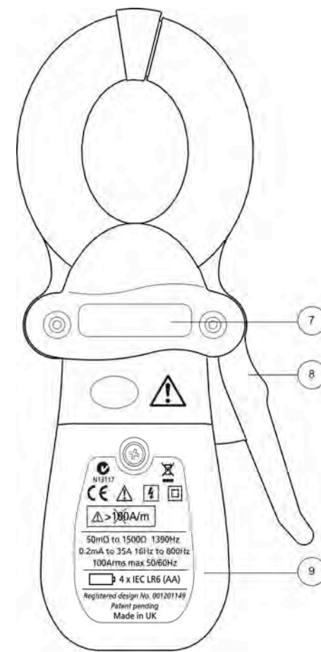
Figure 2: DET14C / DET24C Instrument Rear View
