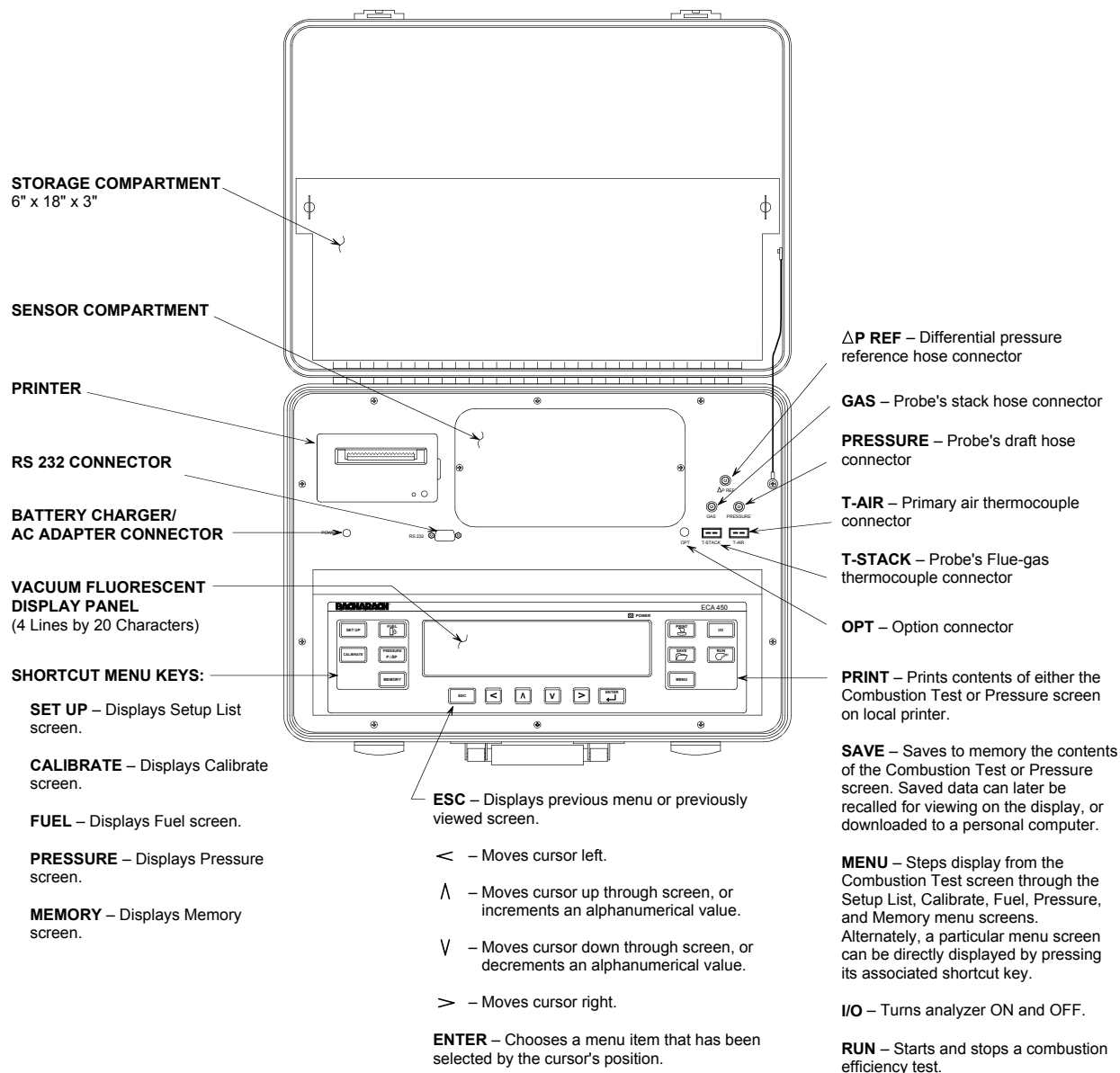
Figure 1-1. ECA 450 Components
