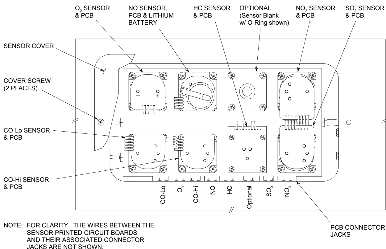
Figure 4-3. Sensor Compartment
