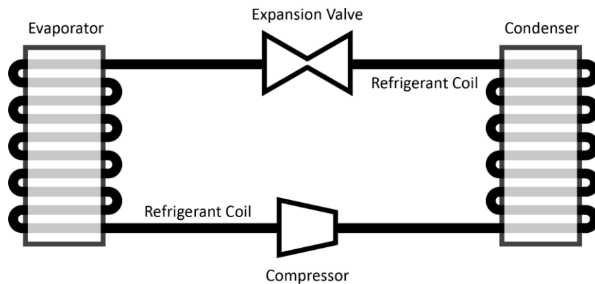
Figure 8. Sample Refrigerant Path for Testing Leaks
