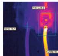
Differential Temperature
