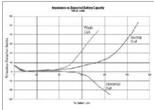
Figure 2. Impedance increases with battery age (and weakness).
